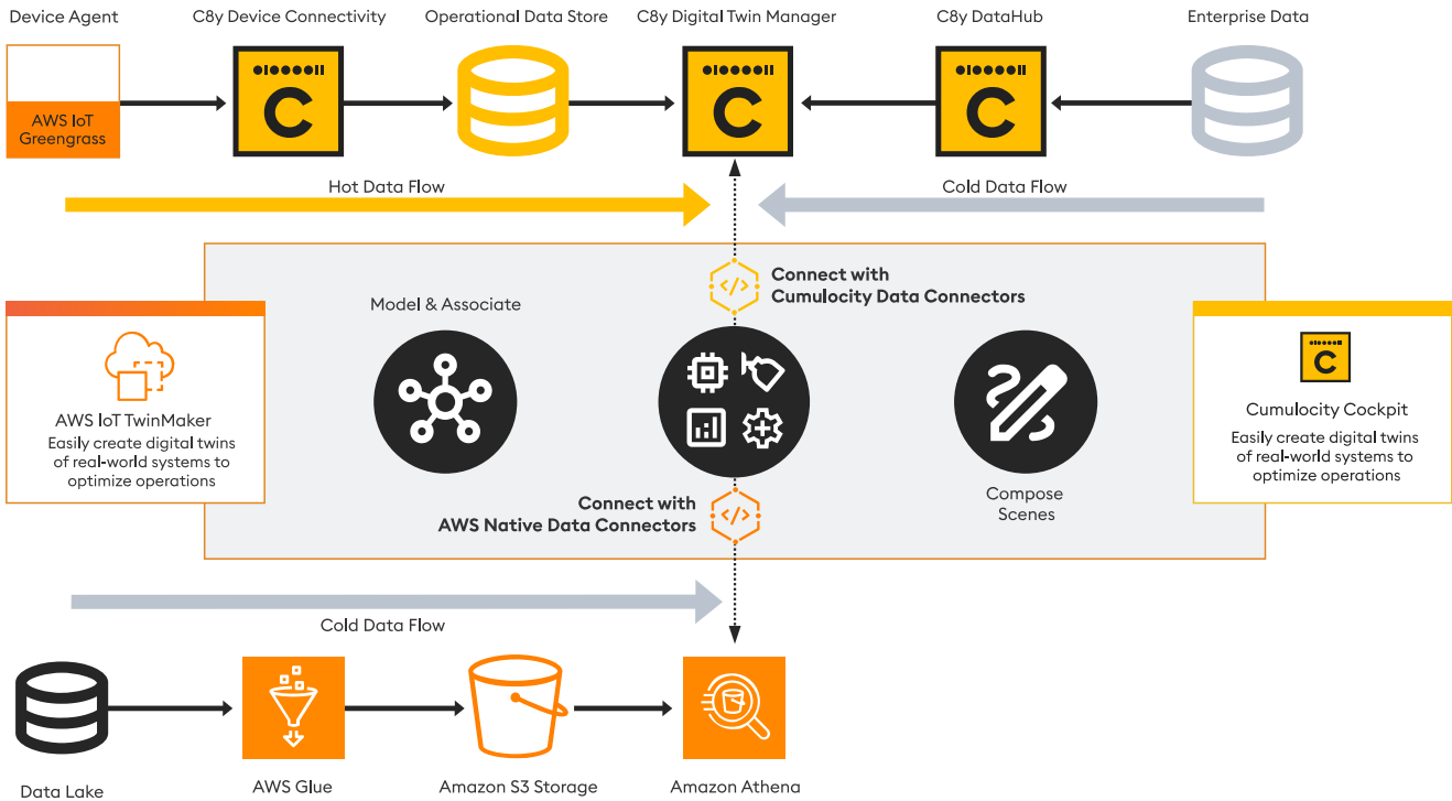
Figure 1. AWS IoT TwinMaker
