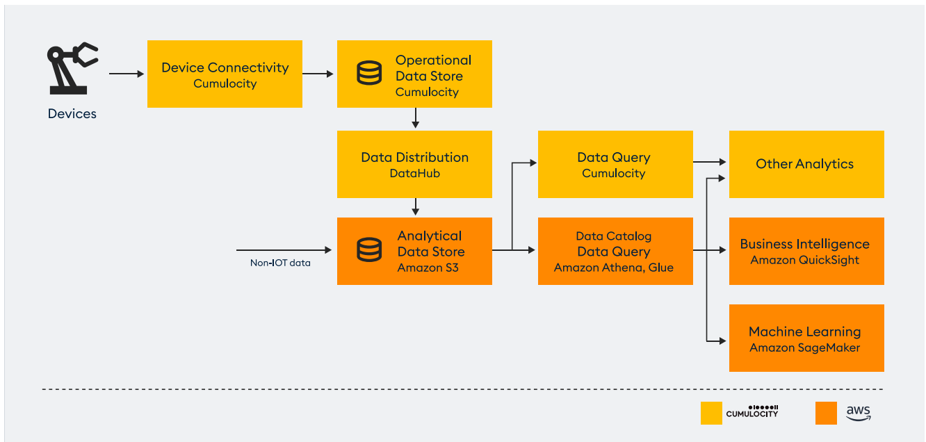
Figure 4. Data flow from device to analytics solution
