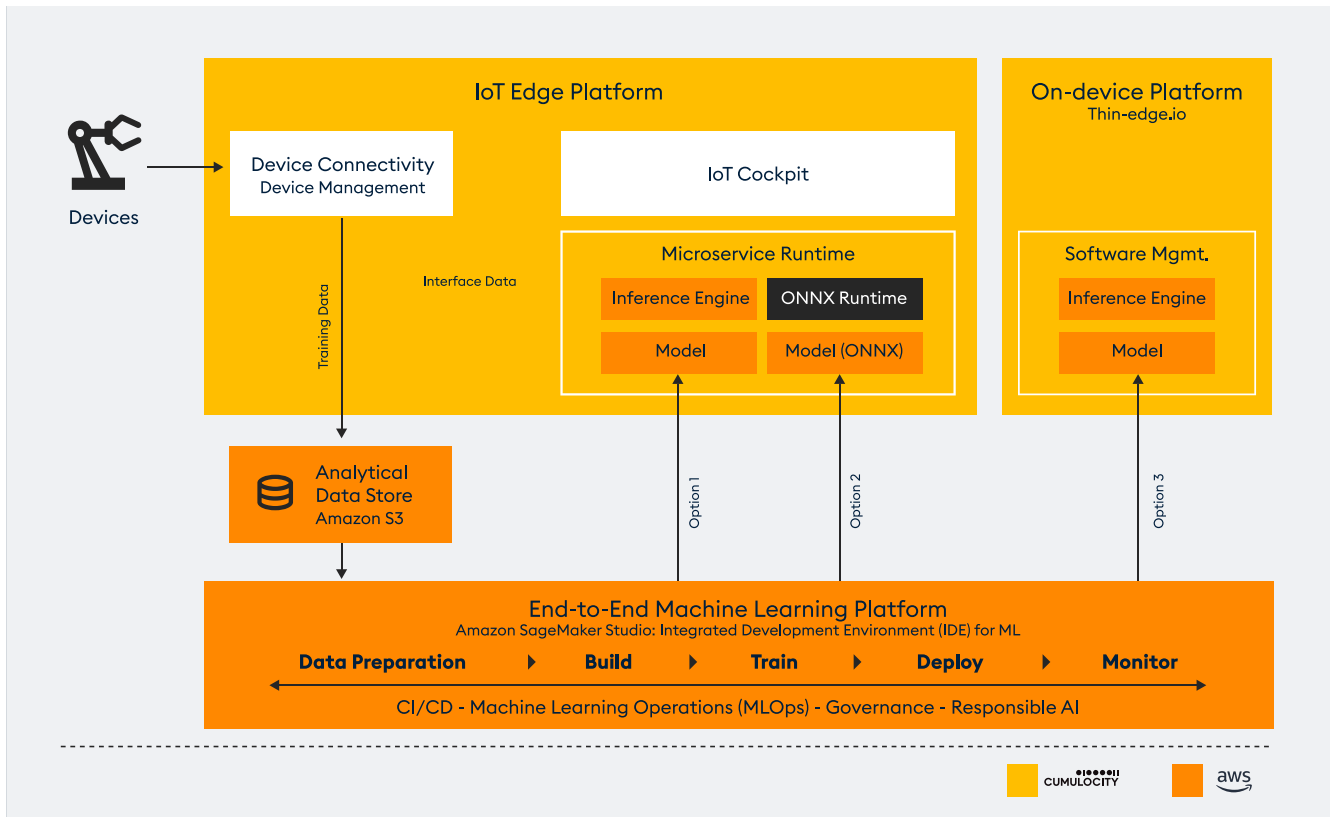
Figure 6. Deploying ML models on the Edge and onto devices
