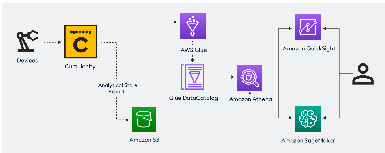
Figure 3. Analytics solutions using Cumulocity and AWS product suite
