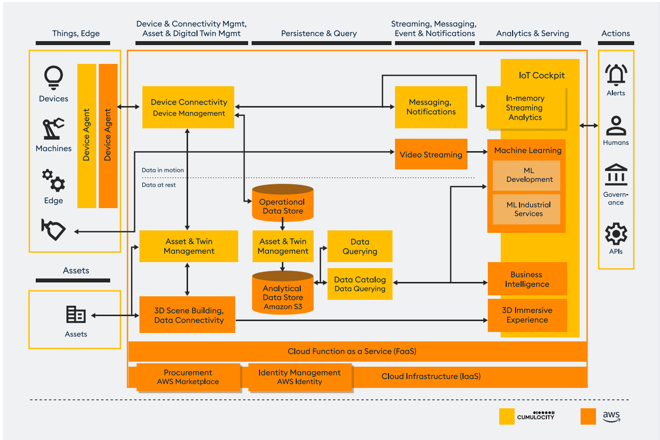
Figure 11. Joint capability architecture showing interaction and data flow between Cumulocity and AWS
