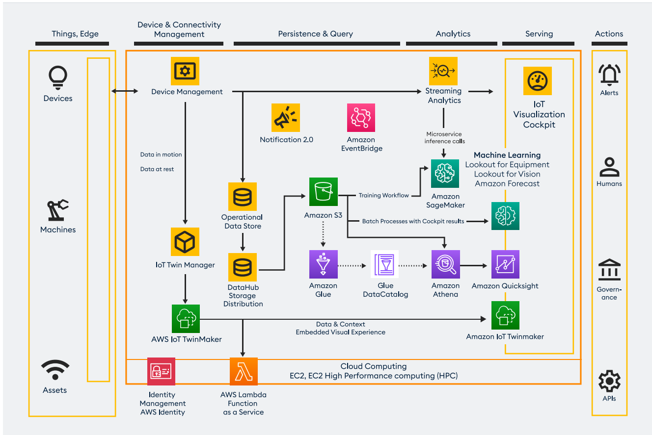
Figure 12. Joint product architecture showing integration points and data flow between Cumulocity and AWS
