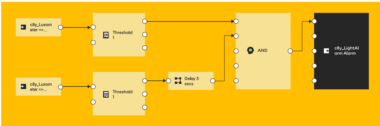
Figure 2. Drag-and-drop composition of streaming analytics solutions with the Analytics Builder
