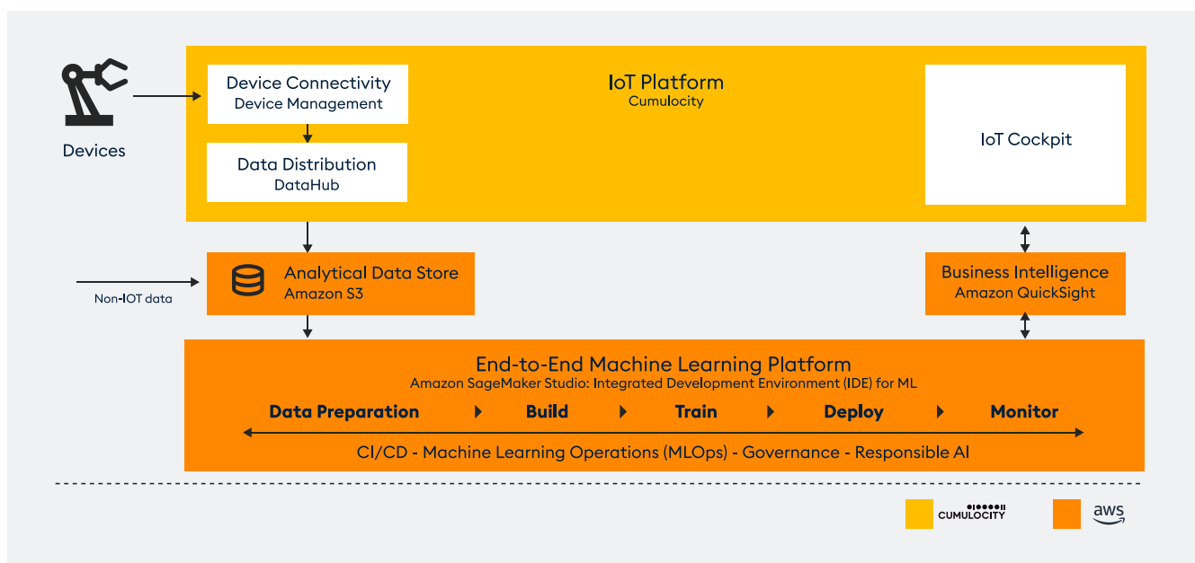
Figure 5. Integrating Cumulocity with Amazon SageMaker
